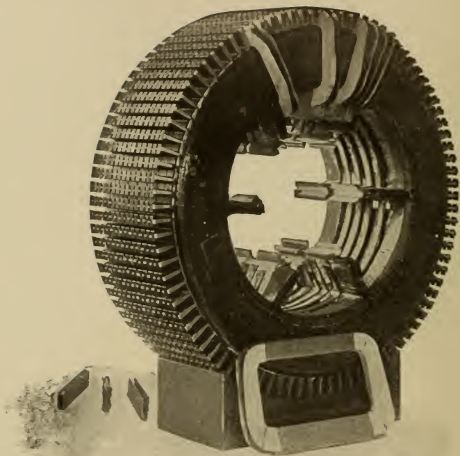
Fig. 13. ARMATURE CORE.
